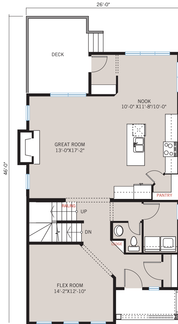
MAIN FLOOR (1,060 SQ FT)
